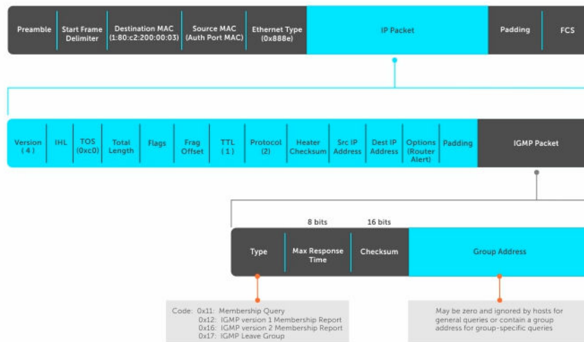
Figure 37. IGMP Messages in IP Packets
